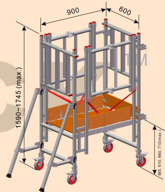
LOYAL Deck Assembly
